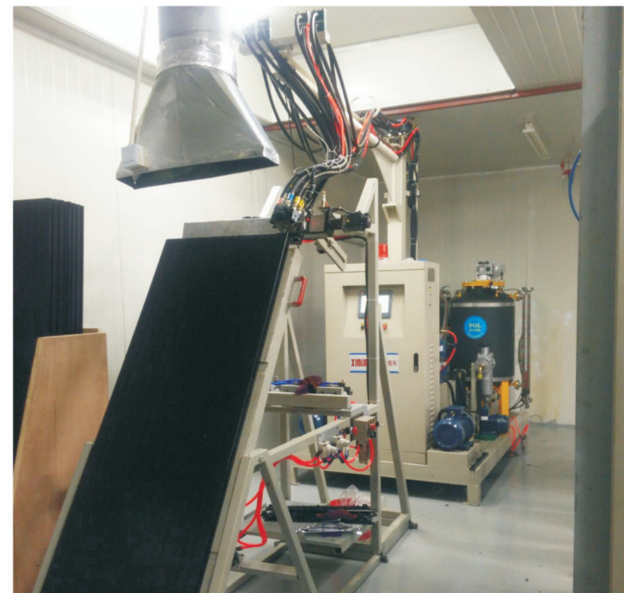
伺服电机控制混合头移动发泡 Servo motor control foam mixing head movement
