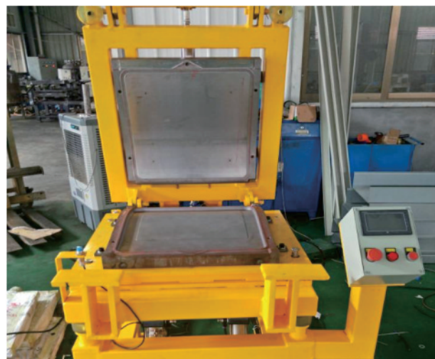
自结皮椅子发泡模架 Self-skinning chair foaming formwork
